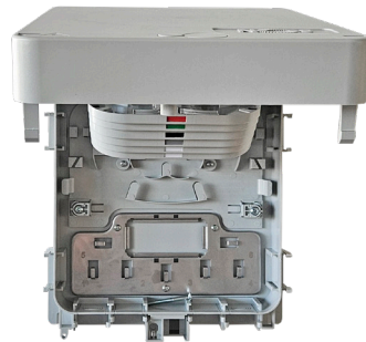
FTB CONNECT lid - self supported at 90 and 130 degrees
