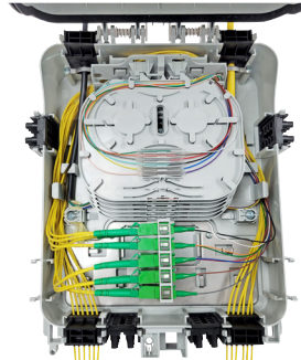
FTB CONNECT - top and bottom access ports
