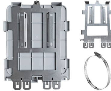
FTB CONNECT (rear view) with pole mounting kit
