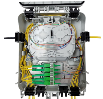
FTB CONNECT - side and bottom access ports
