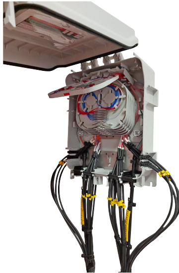
FTB CONNECT using 4 bottom and 2 side access ports. Safety screw restricting operator B from accessing operator A trays
